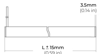
SIDE FEED
