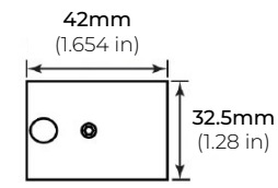
CEILING MOUNT
