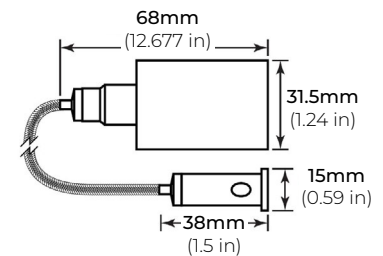
SUSPENDED PENDANT
