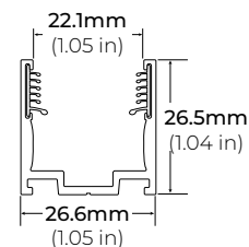
LNT85-HB-AC2/ AC39
