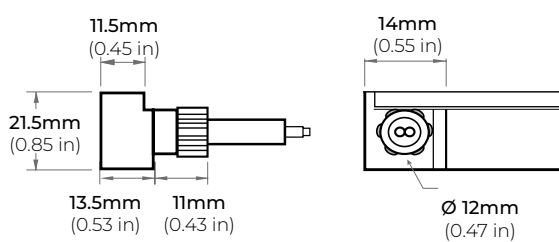
SFR SIDE FEED RIGHT
