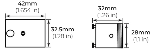
MOUNT CAP 2
