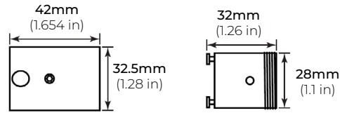
MOUNT CAP 1
