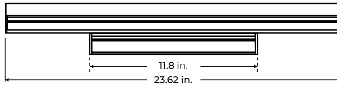
LPX120-24
