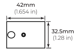
CEILING MOUNT
