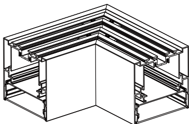
ALP-350TL-L90 L connector (SIDE)
