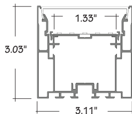
ALP-310N SUSPENSION MOUNT LENGTHS 48" and 96" LENS Frosted FINISH Anodized Aluminum
