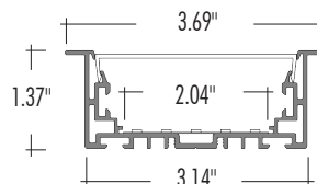
ALP-330RN RECESSED MOUNT LENGTHS 48" and 96" LENS Frosted FINISH Anodized Aluminum
