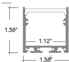
ALP-140 SURFACE / SUSPENSION LENGTHS 49.25" , 98.5" LENS Frosted FINISH Anodized Aluminum
