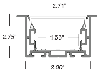
ALP-230RN RECESSED MOUNT LENGTHS 49.25" and 98.5" LENS Frosted FINISH Anodized Aluminum
