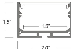
ALP-160 SURFACE / SUSPENDED LENGTHS 49.25" and 98.5" LENS Frosted FINISH Anodized Aluminum
