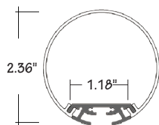
ALP-245 SUSPENSION MOUNT LENGTHS 49.25" and 98.5" LENS Frosted FINISH Anodized Aluminum
