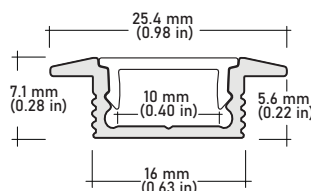
ALP-20R Recessed LENGTHS 49.25" | 98.5" LENS Frosted FINISH White | Black | Silver
