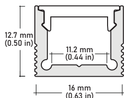
ALP-60 Surface LENGTHS 49.25" | 98.5" LENS Frosted FINISH White | Black | Silver
