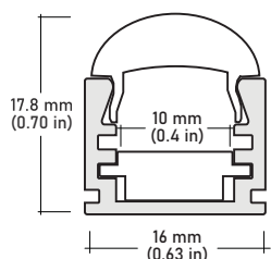
ALP-65 Surface LENGTHS 49.25" | 98.5" LENS Frosted FINISH Silver OPTICS 10° | 30° | 60°
