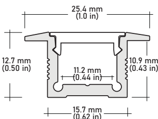
ALP-60R Recessed LENGTHS 49.25" | 98.5" LENS Frosted FINISH White | Black | Silver
