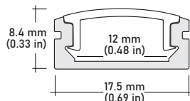
ALU-SF Surface LENGTHS 39 3/8" | 78 7/8" | 98" LENS Clear, Frosted FINISH Silver | Black
