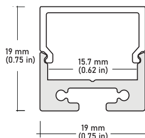
ALP-80 Surface, Suspended LENGTHS 49.25" | 98.5" LENS Frosted FINISH Silver
