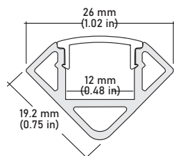
ALU-CN Surface, Corner LENGTHS 39 3/8" | 78 7/8" | 96" LENS Clear, Frosted FINISH Silver | Black
