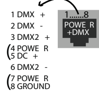
OUTPUT DMX UNIVERSE #1 & #2
