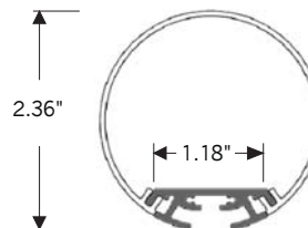
ALP-245 | SUSPENDED MOUNT
