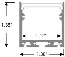
ALP-140 | SURFACE OR SUSPENDED MOUNT
