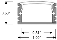
ALU-DS100 | SURFACE MOUNT
