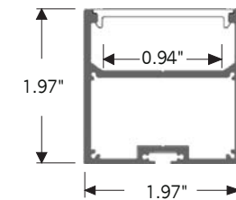
ALP-200 | SURFACE OR SUSPENDED MOUNT
