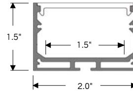
ALP-160 | SURFACE OR SUSPENDED MOUNT
